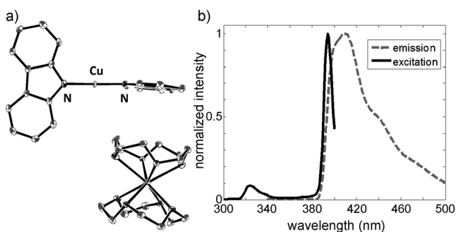
Figure 1. [\text{Li}(\text{[12]crown-4})_2][\text{Cu}(\text{carbazolide})_2] ( 5 ): a) X-ray structure (thermal ellipsoids drawn at 50% probability and H atoms omitted for clarity). b) Excitation (emission wavelength: 410 nm) and emission (excitation wavelength: 325 nm) spectra in \text{CH}_3\text{CN} .
